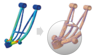
Extract mesh data from the analysis result (Preserving Residual stress)
